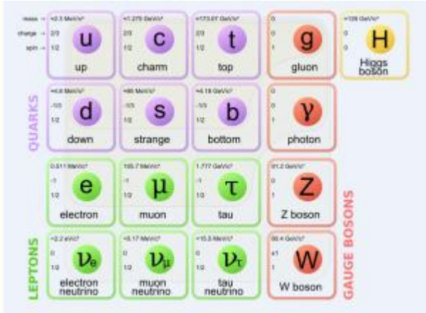
Standard Particle Model
